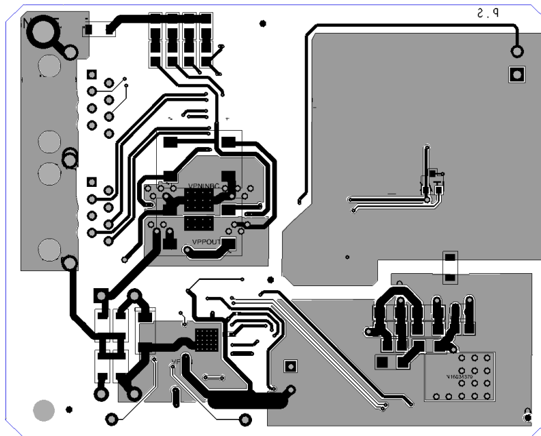
Figure 16: Bottom Layer
