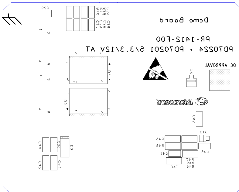
Figure 17: Bottom Silk
