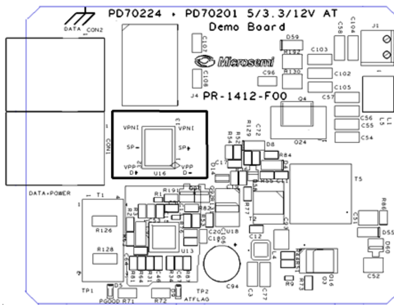
Figure 19: Top Silk
