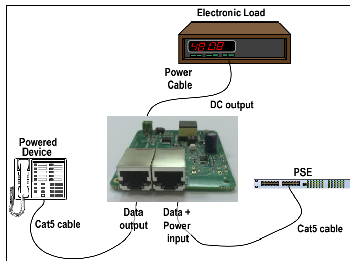
Figure 6: Test Setup
